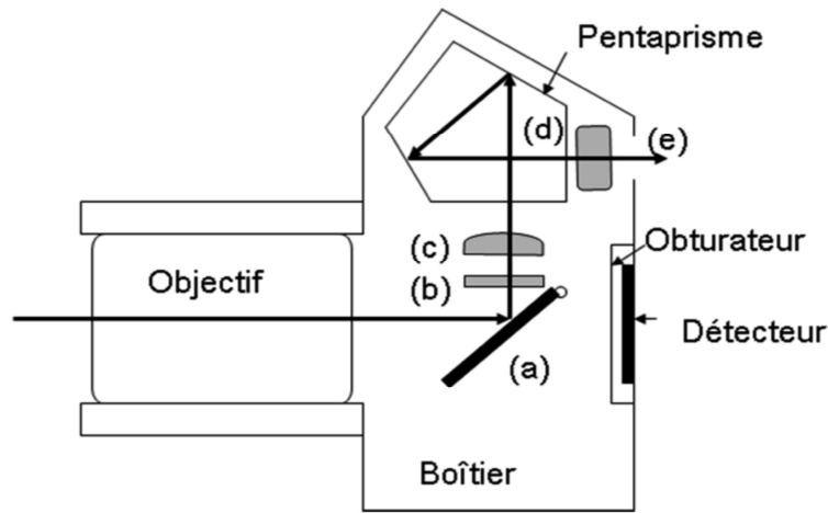
Figure 1 : appareil photo
